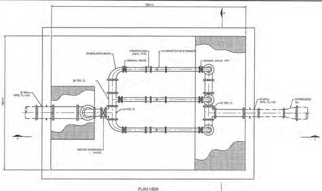
PLAN VIEW
